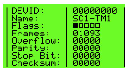
Obr. 2.6 Menu Overview
