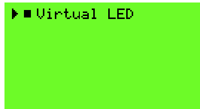
Obr. 2.4 Menu Settings
